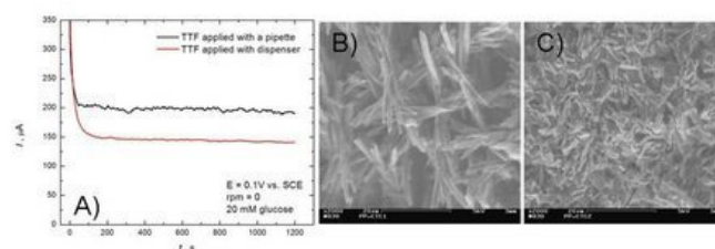
Figure 1: The influence of the CTC morphology on the glucose oxidation activity. A) Chronoamperograms of the different anodes in presence of glucose; SEM images of CTC when TTF solution was applied with B) pipette and C) dispensing robot.
