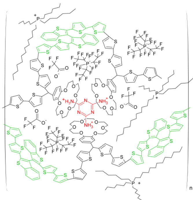
Scheme. Excerpt of structural formula of the MIP-melamine film.
