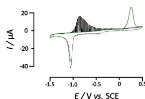
Figure 1. Comparison of the photocatalysed oxidation (black) and dark (green) voltammogram for the Rhodamine B base at 0.01 \text{V/s}^{-1} ; 16 nl deposit, 0.28 M (Rhodamine B : PPP).
