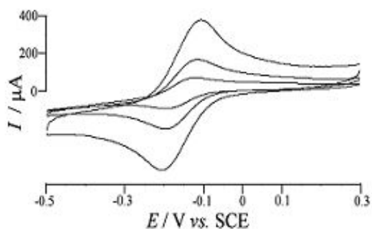
Figure 1: Reversible cyclic voltammograms of 1 mM \text{Ru}(\text{NH}_3)_6^{3+} in 0.1 M KCl at a \text{MoSe}_2 electrode at potential scan rates 0.01, 0.05, and 0.2 \text{ V s}^{-1} .
