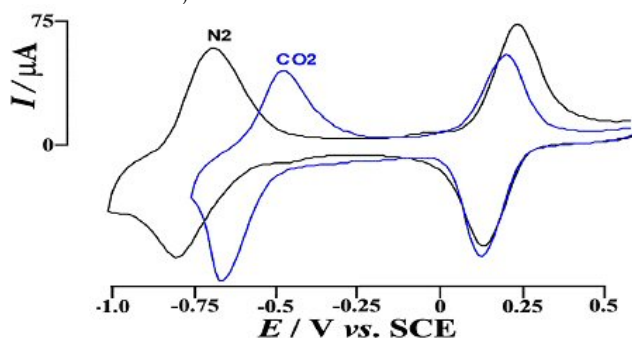
Figure 1 Cyclic voltammogram at 0.05 V s -1 for the oxidation/reduction of 80 nL deposit of a solution of CoPc (84 mM) in 4-(3-phenylpropyl)pyridine, immobilized onto a 4.9 mm diameter basal plane pyrolytic graphite electrode, and immersed in 0.1 M NaClO 4 , in the absence and presence of carbon dioxide.
